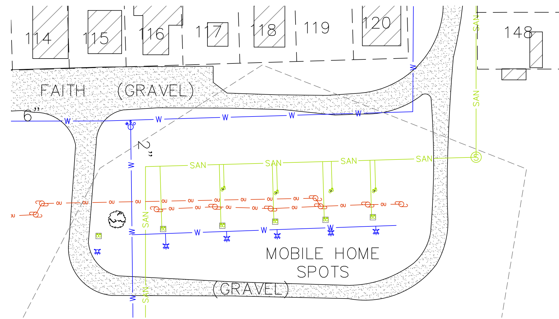
ENLARGED MOBILE HOME SITE SCALE: 1" = 40'
