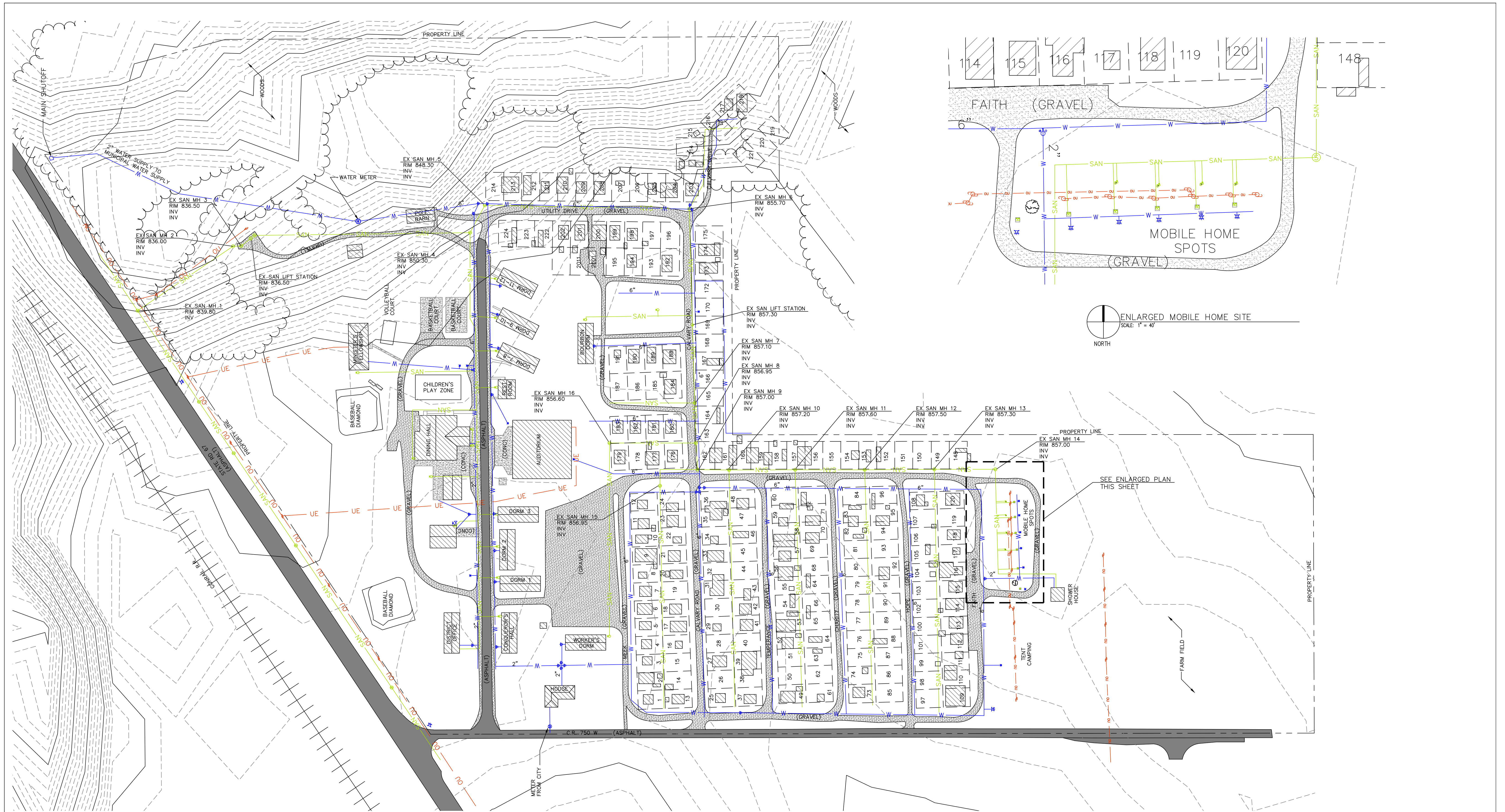
EXISTING UTILITIES SITE PLAN SCALE: 1" = 100'
